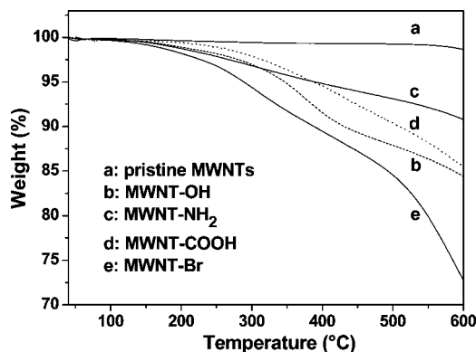
Figure 2. TGA curves of (a) pristine MWNTs, (b) MWNT-OH, (c) MWNT- \text{NH}_2 , (d) MWNT-COOH, and (e) MWNT-Br.
