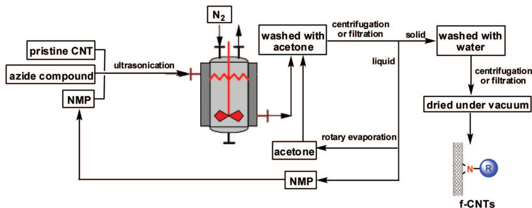
Figure 1. Flowchart for the large-scale production of f-CNTs.
