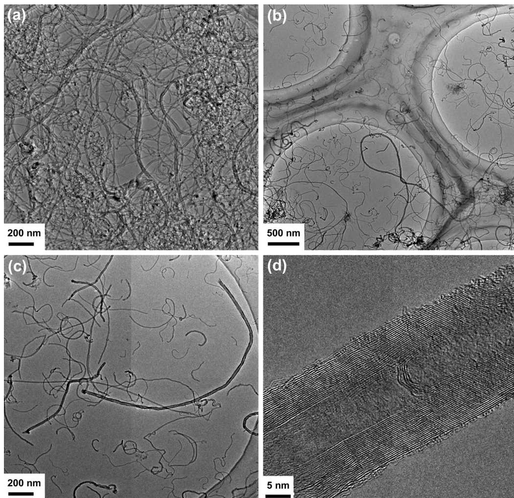
Figure 6. Representative TEM images of p-MWNTs (a) and MWNT-OH (b–d). Other f-MWNTs showed TEM images similar to those of the MWNT-OH.
