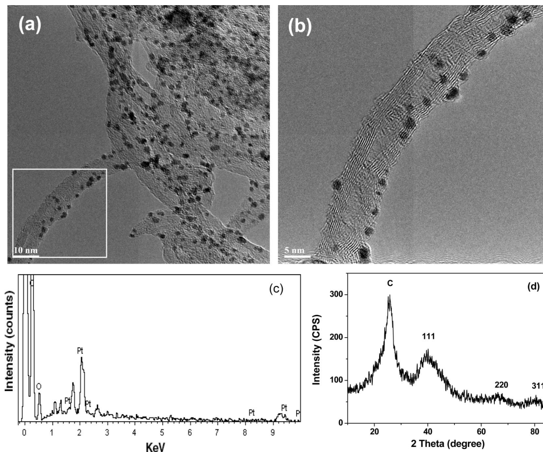
Figure 8. TEM images (a, b), EDS spectrum (c), and XRD pattern (d) of Pt/MWNT-COOH nanohybrids.
