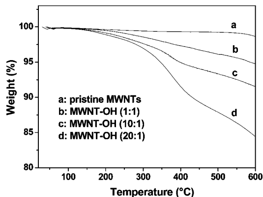
Figure 3. TGA curves of pristine MWNTs (a) and MWNT-OH prepared with different 2-azidoethanol/MWNT mass feed ratios of 1:1 (b), 10:1 (c), and 20:1 (d).
