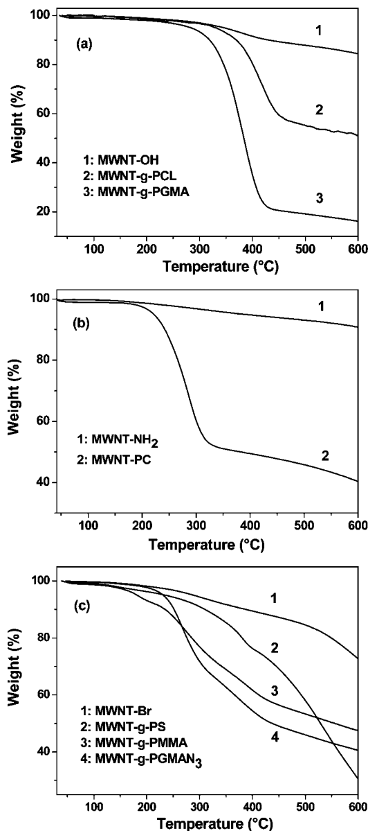
Figure 7. TGA curves of functionalized MWNTs.
