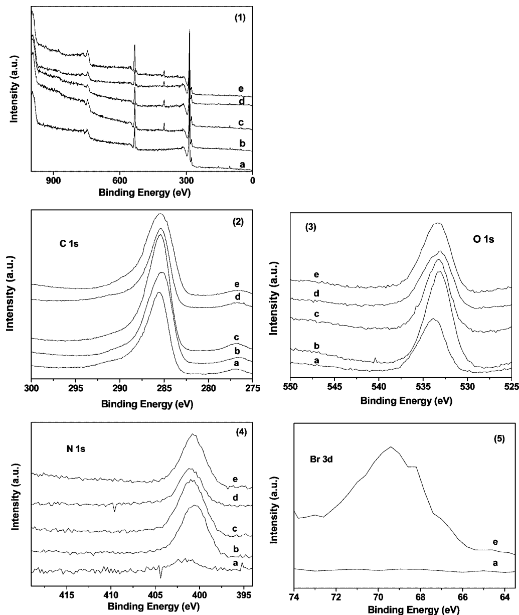
Figure 5. XPS spectra of (a) p-MWNTs, (b) MWNT-OH, (c) MWNT-NH 2 , (d) MWNT-COOH, and (e) MWNT-Br: (1) survey of the spectral region from 0 to 1000 eV, (2) the carbon 1s region, (3) the oxygen 1s region, (4) the nitrogen 1s region, and (5) the bromine 3d region.
